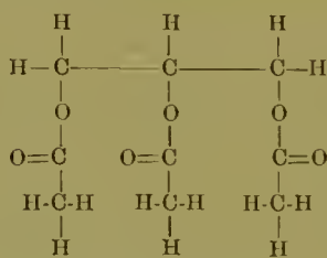
C_3H_5O_3(C_2H_3O)_3 Triacetylglycerinäther (Triacetin) (Neutrales Fett).
